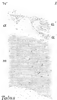
Section transverse to Glen Roy and nearly opposite Glen Glaster.
